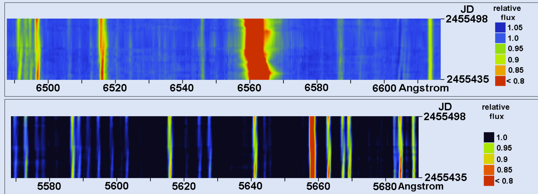
Contour plot showing line doubling (C Buil eShel, 0.6A resolution)
